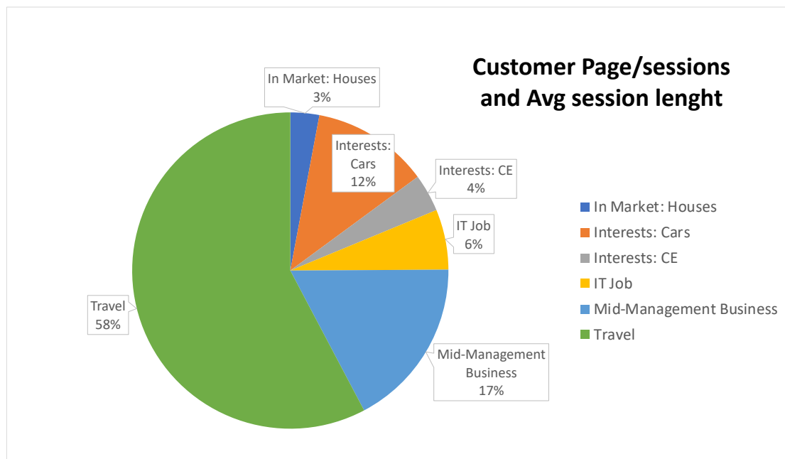
Fig.7 Customer Page/sessions
